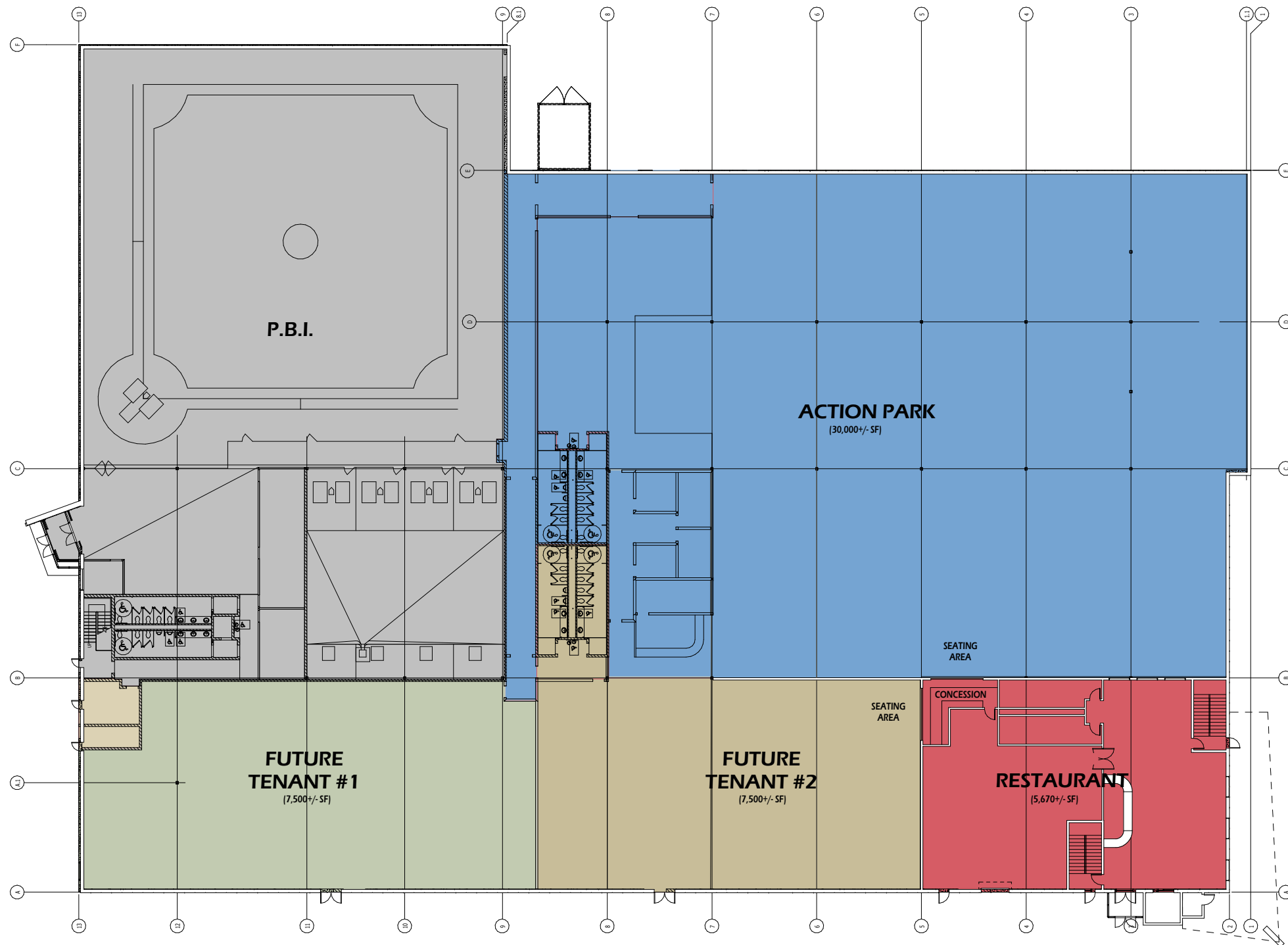
① OVERALL FLOOR PLAN 1/16" = 1'-0"
